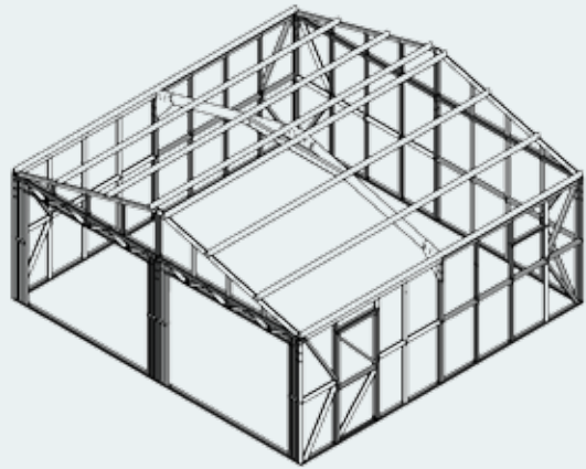
Option 2: As per standard gable with 3m wide full length open awning
