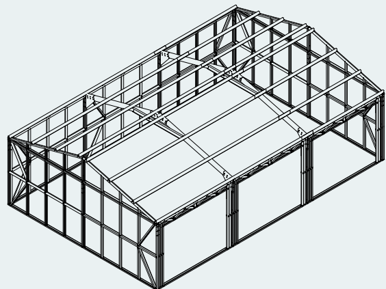
Option 4: Standard gable with side entry access up to 12m long allowing you the choice of bays
